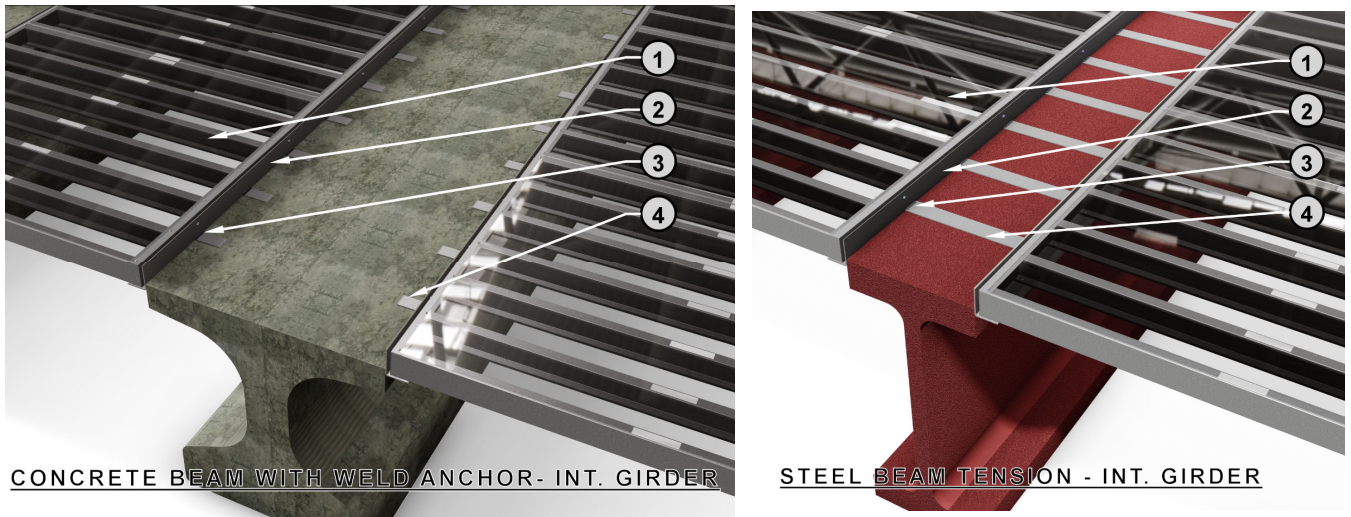
1 – Structural Steel Joist, 2 – Steel Angle Support, 3 – Fillet Weld, 4 – Weld Anchor or Weld Strap
