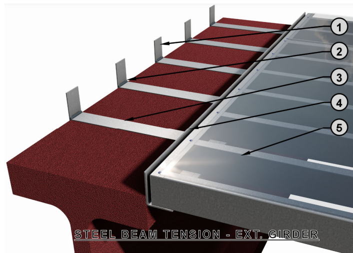
1 – Clip Angle, 2 – Fillet Weld, 3 – Strap, 4 – Steel Angle Support, 5 – Transparent Acrylic
